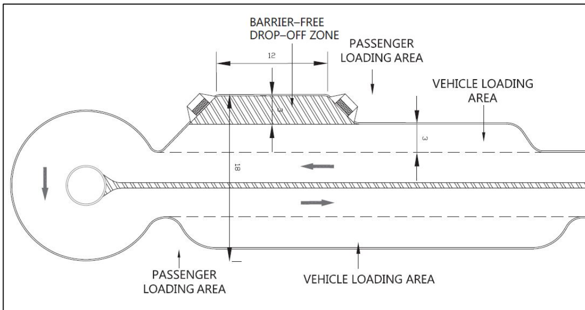
Figure 13-3 Strip Configuration
