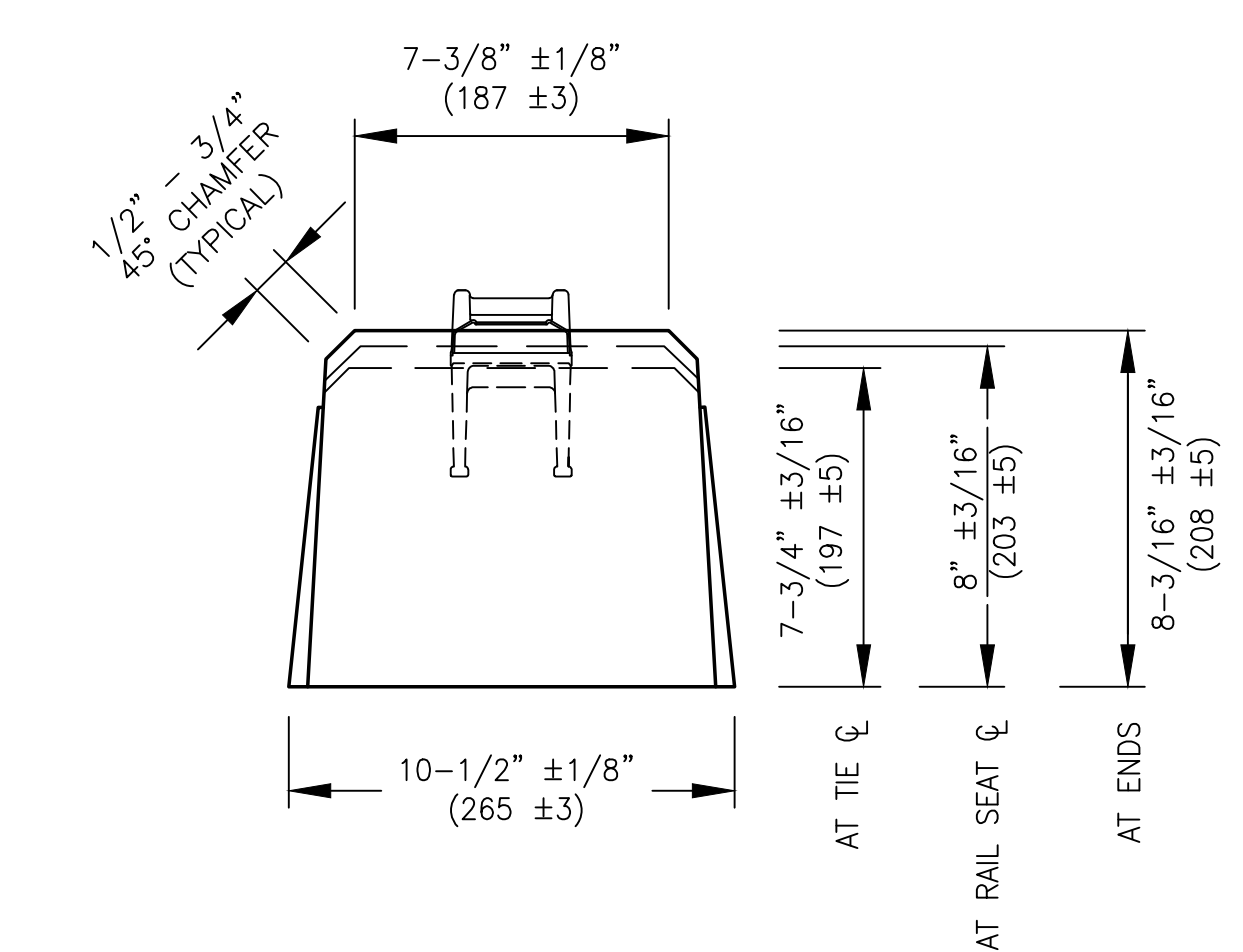
SECTION A
