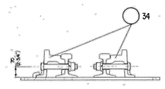
TOE OF FROG ASSEMBLY
