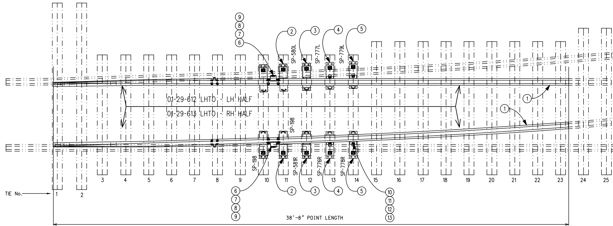
LEFT HAND TURNOUT
