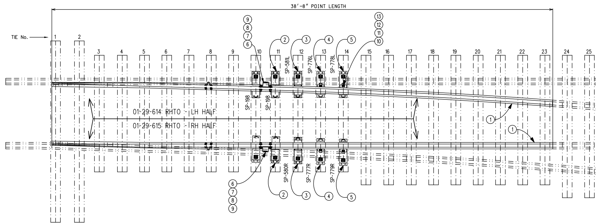
RIGHT HAND TURNOUT
