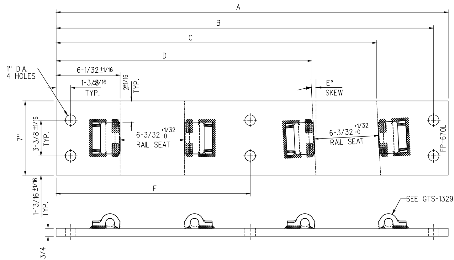
PANDROL SHOULDER DETAIL
