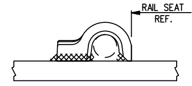
PANDROL SHOULDER DETAIL
