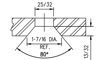
COUNTERSINK DETAIL
