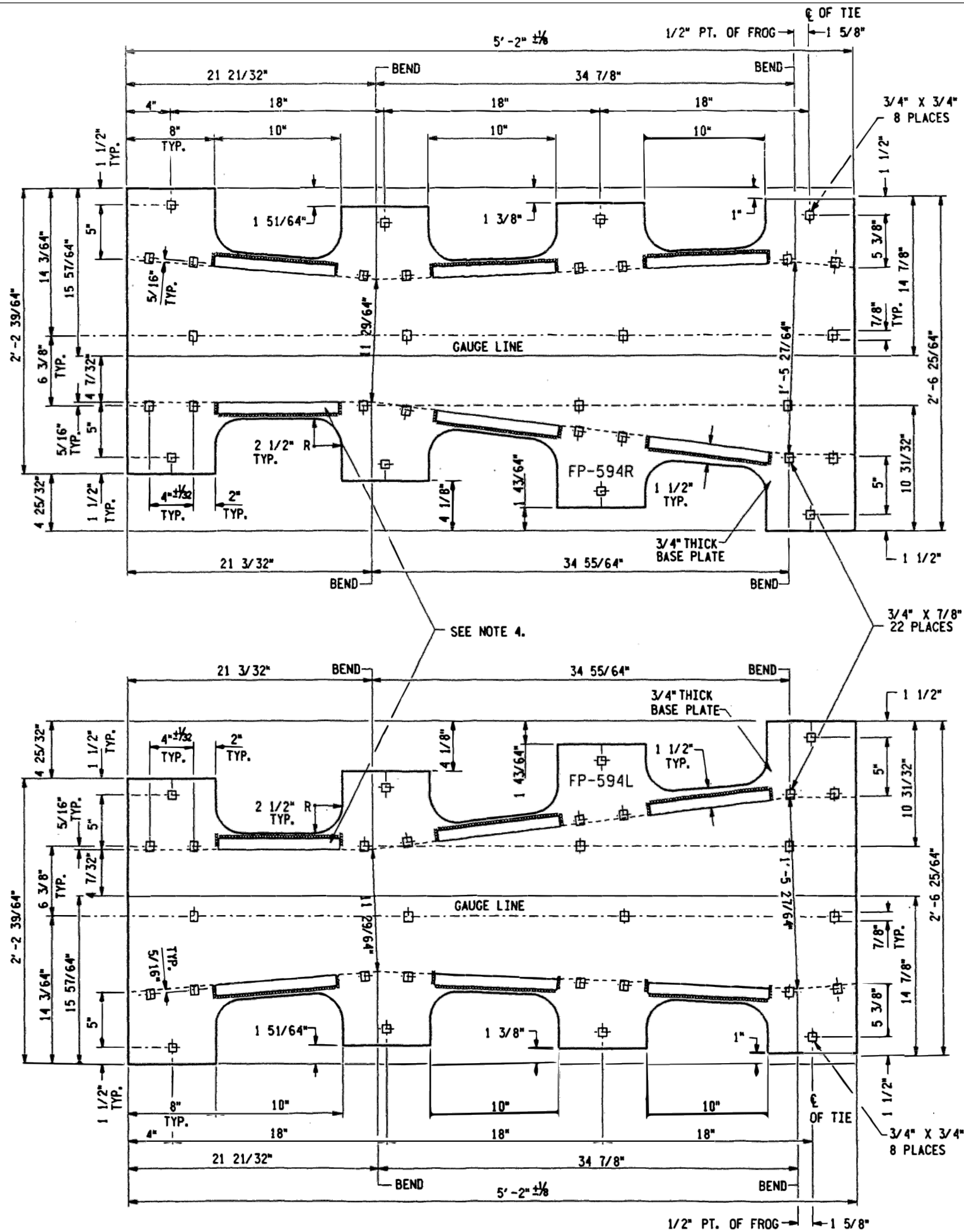
FROG BASE PLATE FP-594R
