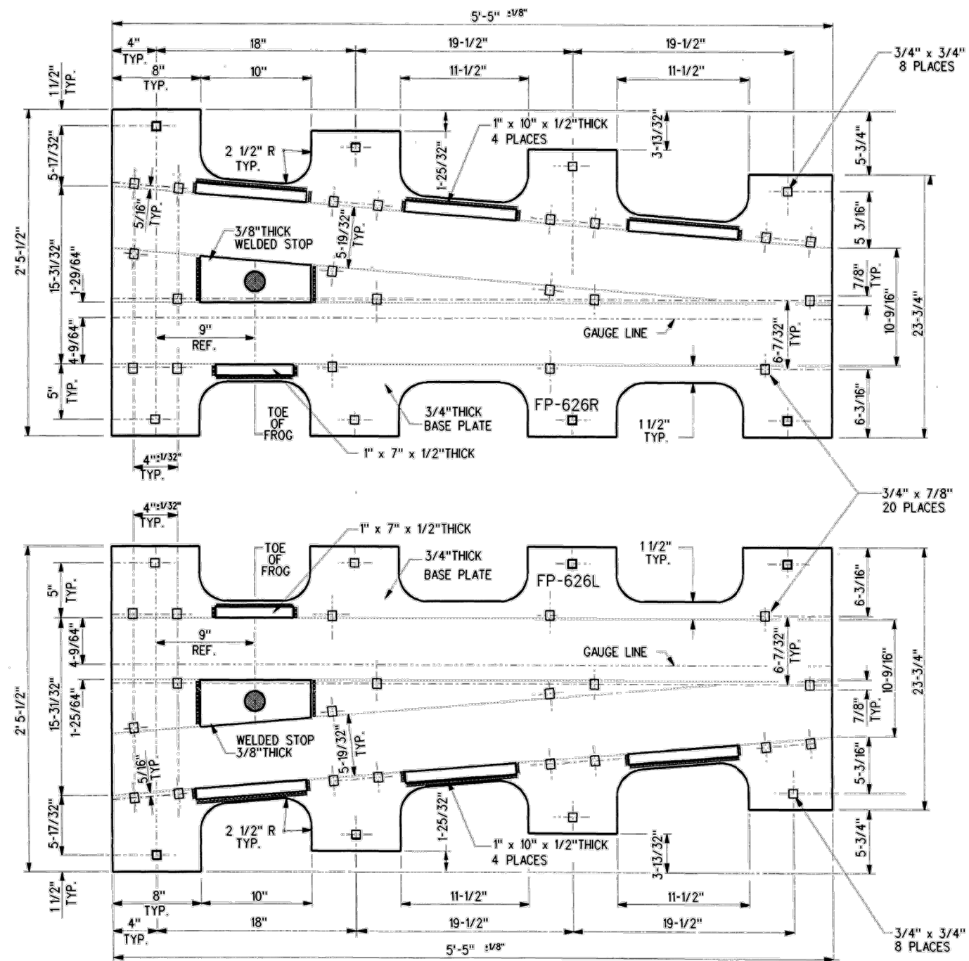
FROG BASE PLATE FP-626R
