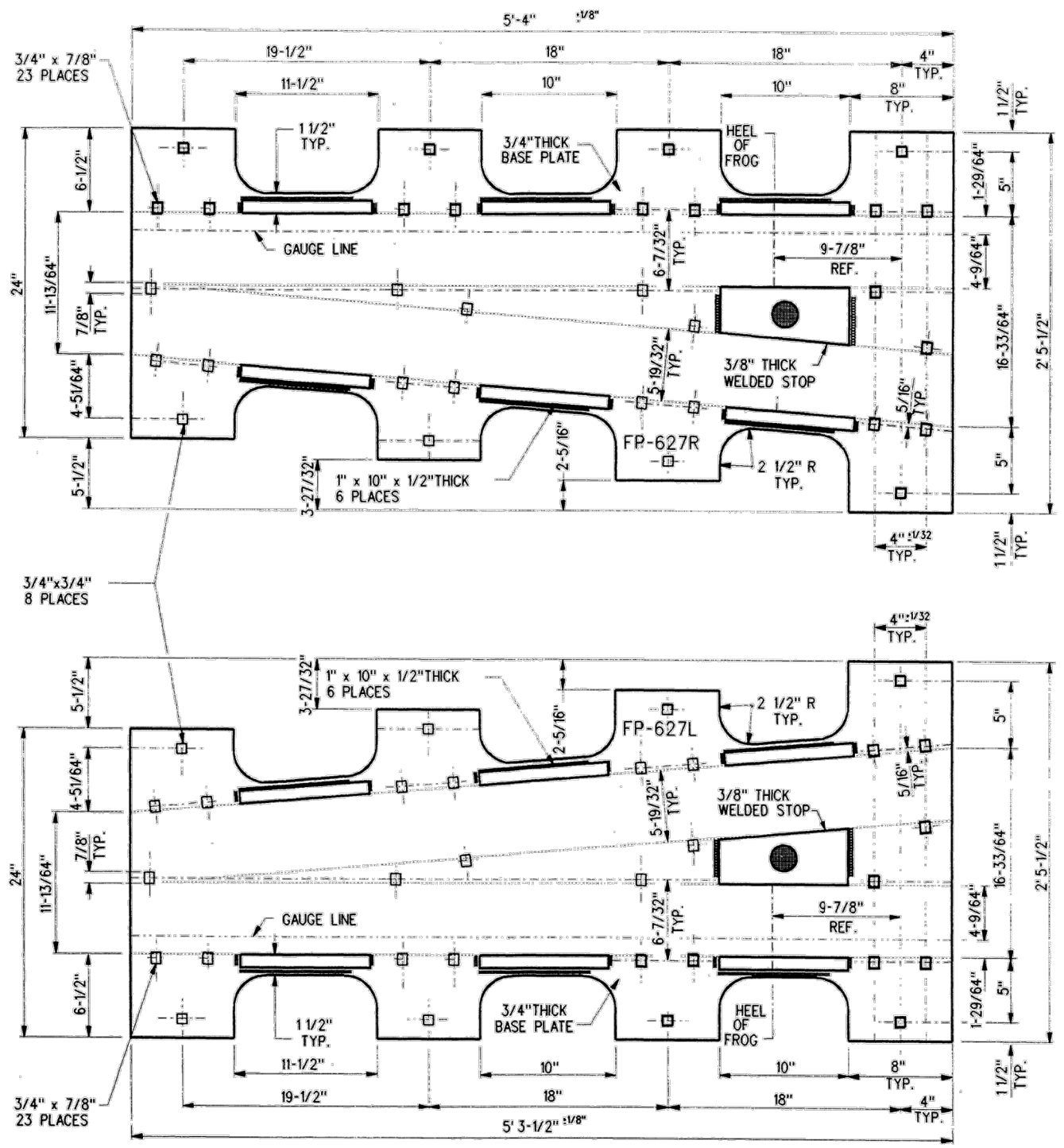
FROG BASE PLATE FP-627R
