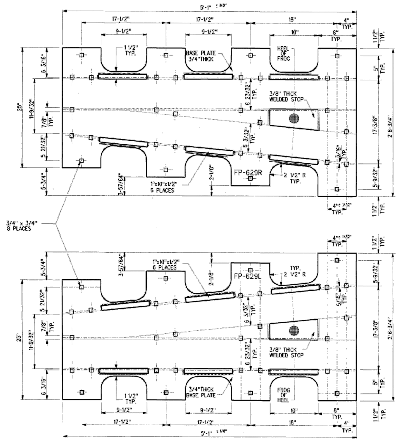
FROG BASE PLATE FP-629R
