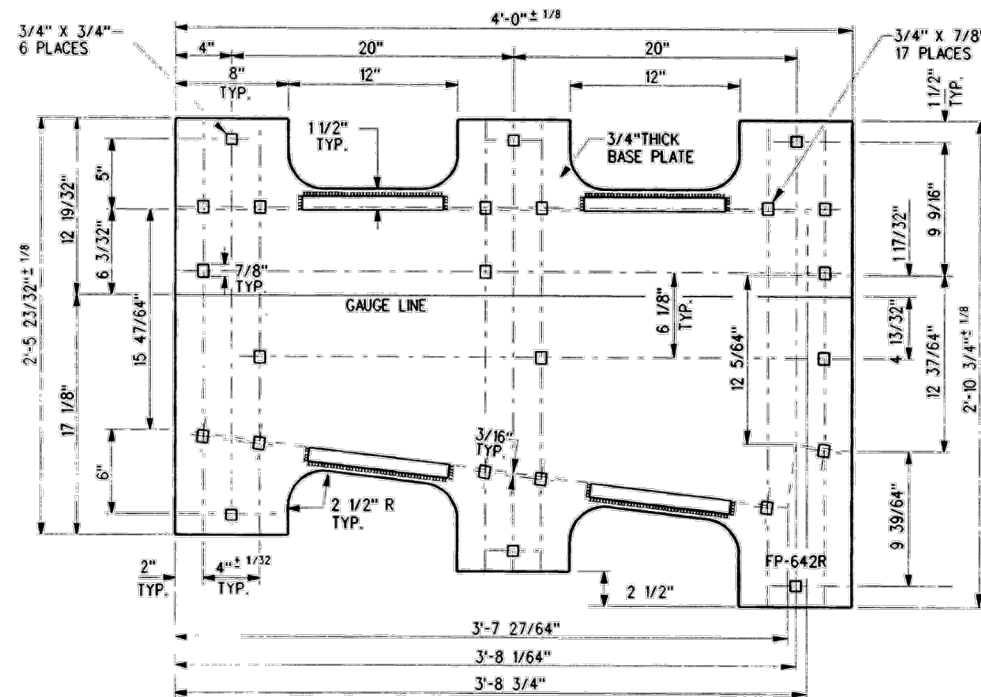
FROG BASE PLATE FP-642R
