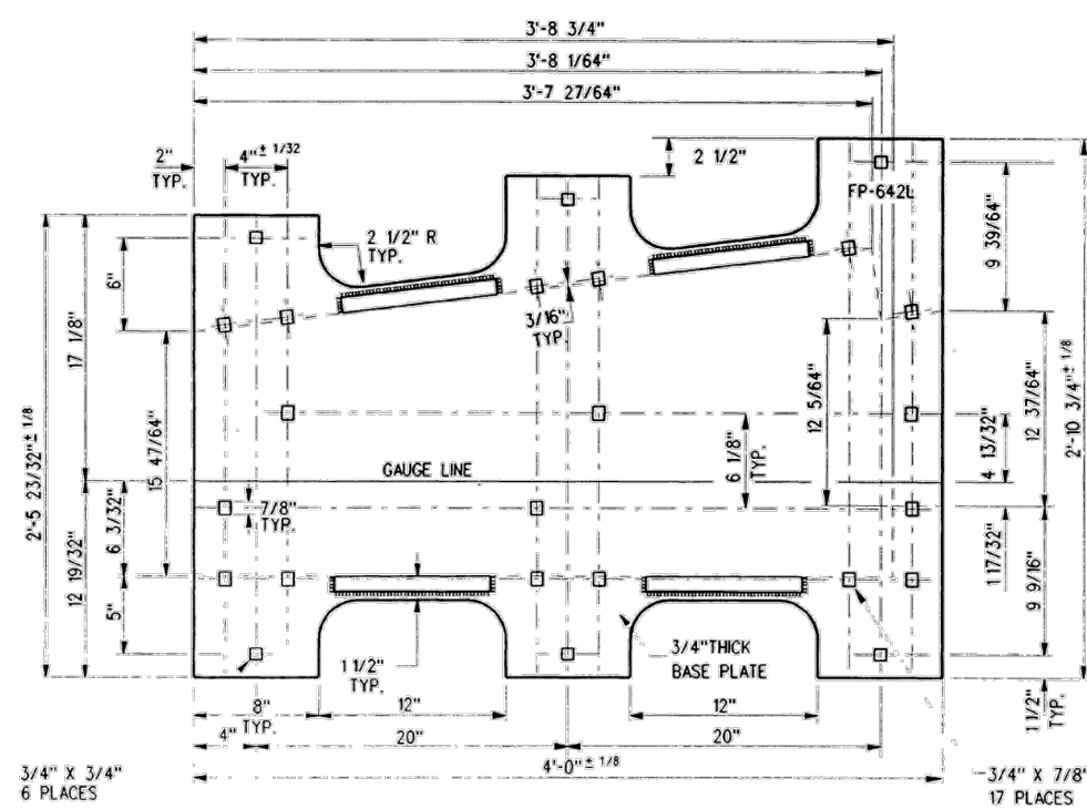
FROG BASE PLATE FP-642L
