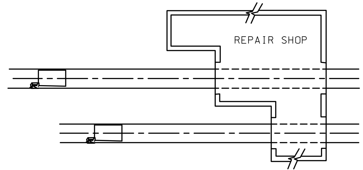
PIT LOCATION DETAIL
