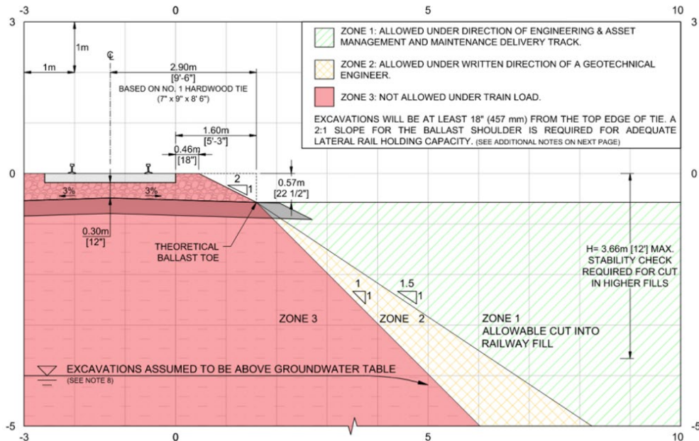
Figure: Appendix W - GO Transit Track Standards [3]
