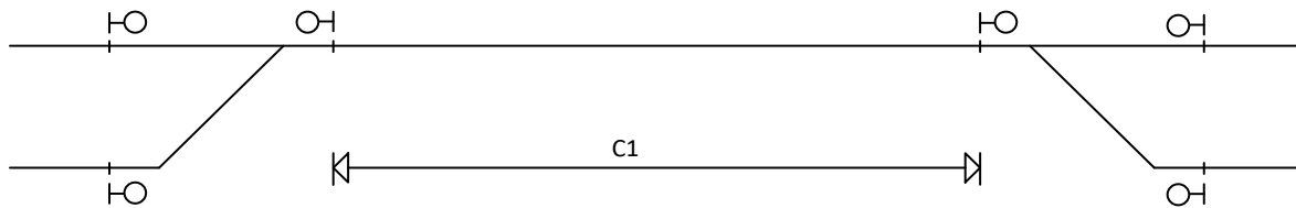
Figure 05 - One-Block Track Indication
