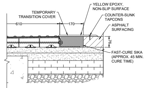
TEMPORARY TRANSITION COVER DETAIL
