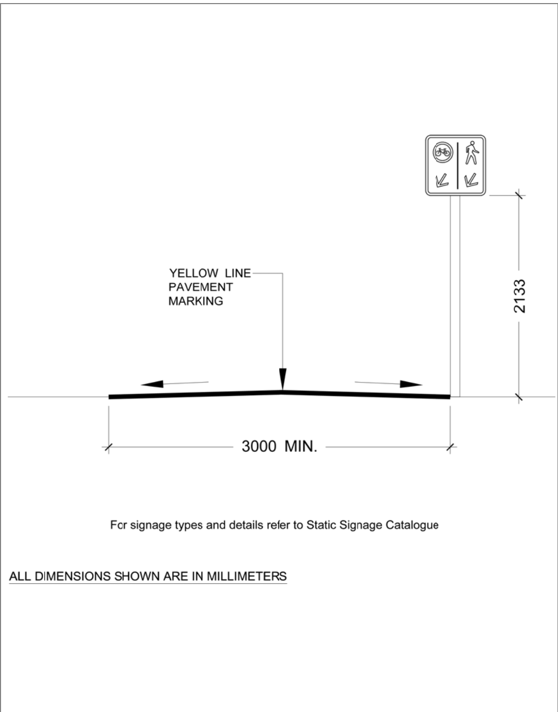
FIGURE: TYPICAL CROSS SECTION FOR SHARED PEDESTRIAN/CYCLIST PATH DESIGN
