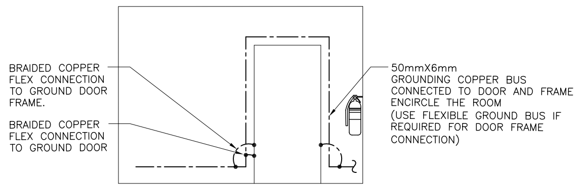
TYPICAL GROUNDING BUS ON WALL 3 E-2001B
